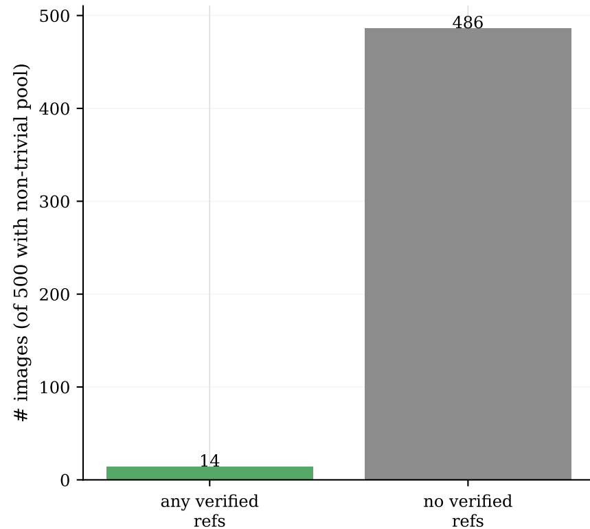
RAG coverage
